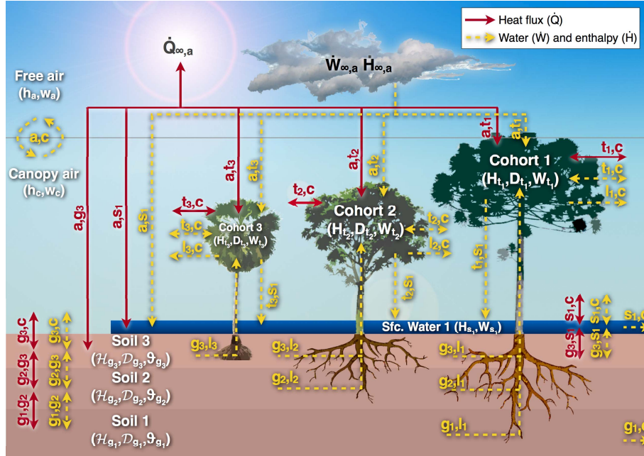
Figure 2. Schematic of the fluxes that are solved in ED-2.2 for a single patch (thermodynamic envelope). In this example, the patch has three cohorts, a single surface water layer, and three soil layers. Letters near the arrows are the subscripts associated with fluxes, although the flux variable has been omitted here for clarity. Solid red arrows represent heat flux with no exchange of mass, and dashed blue arrows represent exchange of mass and associated enthalpy. Arrows that point to a single direction represent fluxes that can only go in one (non-negative) direction, and arrows pointing to both directions represent fluxes that can be positive, negative, or zero.
